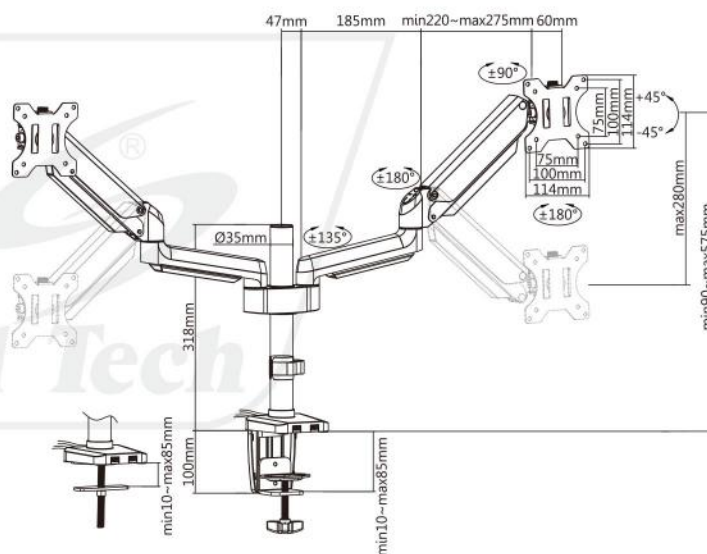
Premium Gas Spring Aluminum Monitor Arm
